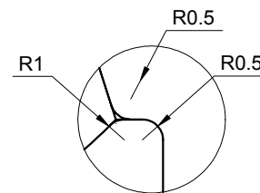
Detail K
